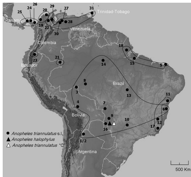
Figure 1 Anopheles triannulatus s.l. sampled localities. The locality numbers correspond to those in Table 1. Black dots represent Anopheles triannulatus s.l., black and white triangles represent An. halophylus and An. triannulatus C type localities, respectively. The map depicts the k = 9 groups yielded by SAMOVA software and supported by AMOVA analysis.
