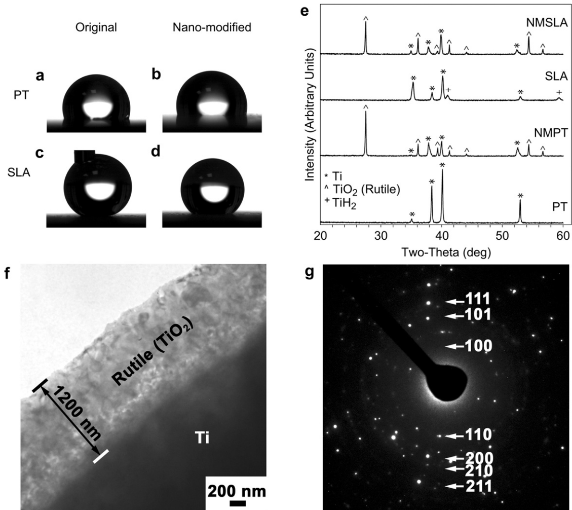
Fig. 5. Surface characterization data of the NM-treated samples, which were oxidized in flowing synthetic air for 90 min at 740 °C, and their controls. (a–d) Optical images of water contact angles on PT, SLA, NMPT, and NMSLA surfaces. The contact angles measured for PT and NMPT samples were similar and smaller than for the SLA and NMSLA samples. (e) X-ray diffraction (XRD) patterns obtained from PT, SLA, NMPT, and NMSLA samples. (f) TEM image of an ion-milled cross-section of an NMPT specimen revealing the compact and conformal oxide layer formed after NM treatment. The average thickness of this oxide scale was 1.2 μm. (g) Selective area electron diffraction pattern obtained from the oxide scale, which was consistent with pure rutile TiO 2 .
