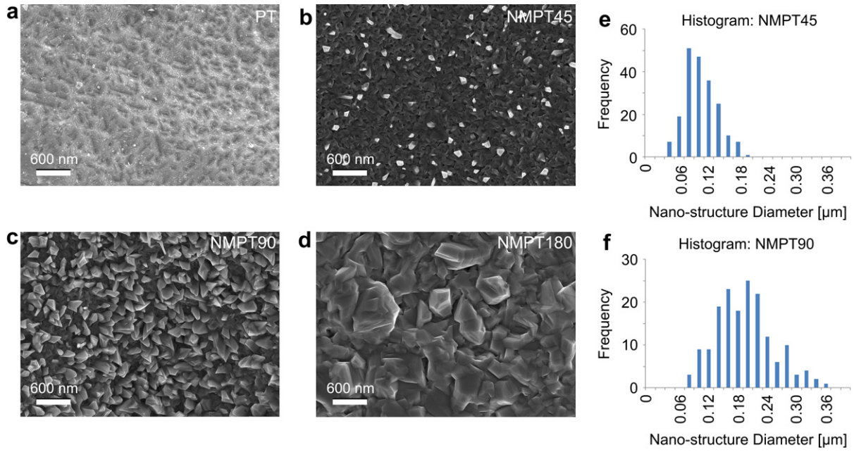
Fig. 2. NM treatment of (a) PT surfaces via oxidation in flowing synthetic air (21% O 2 , 79% N 2 ) at 740 °C for times of: (b) 45 min; (c) 90 min; (d) 180 min. The modification process introduced: (b) nanoscale protuberances with low surface coverage after 45 min; (c) a relatively high density of nanostructures after 90 min; and (d) coarse structures after 180 min. These SEM images are representative of the entire PT Ti disk surfaces. (e, f) Image analyses of SEM images revealing the distribution of diameters of the nanoscale structures formed after 45 min and 90 min, respectively.
