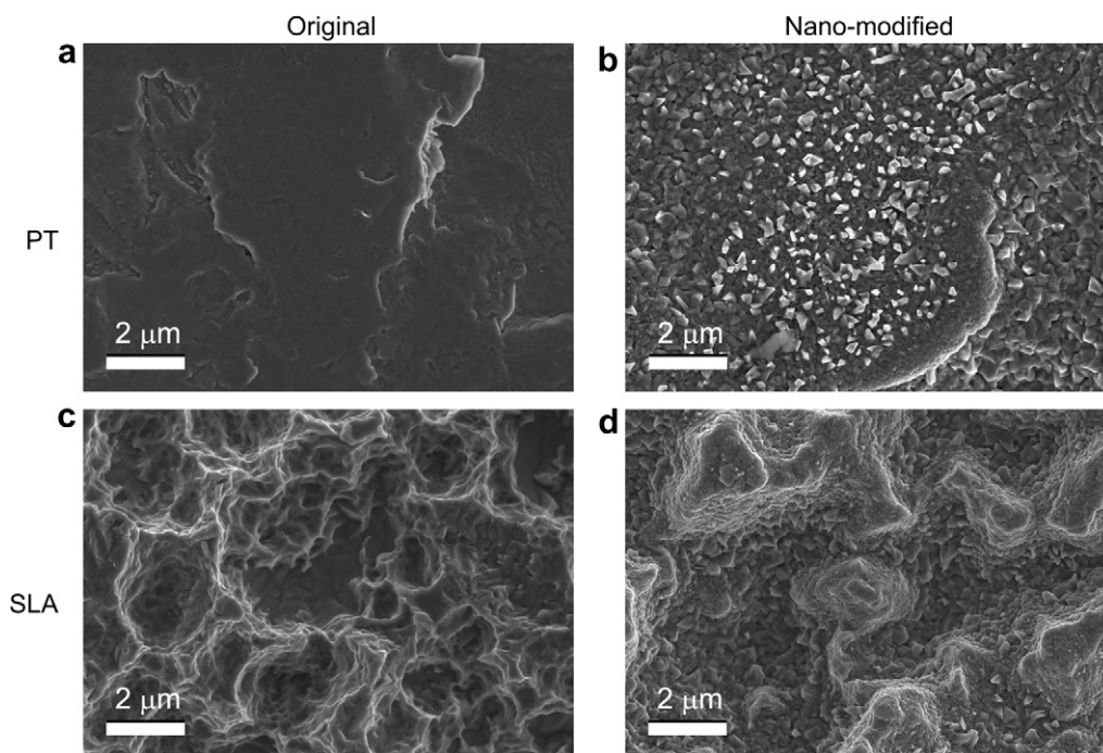
Fig. 4. SEM images of the surface of (a) PT, (b) NMPT, (c) SLA, and (d) NMSLA samples used for further surface characterization and for cell experiments. The NM treatment consisted of oxidation in flowing synthetic air for 90 min at 740 °C.
