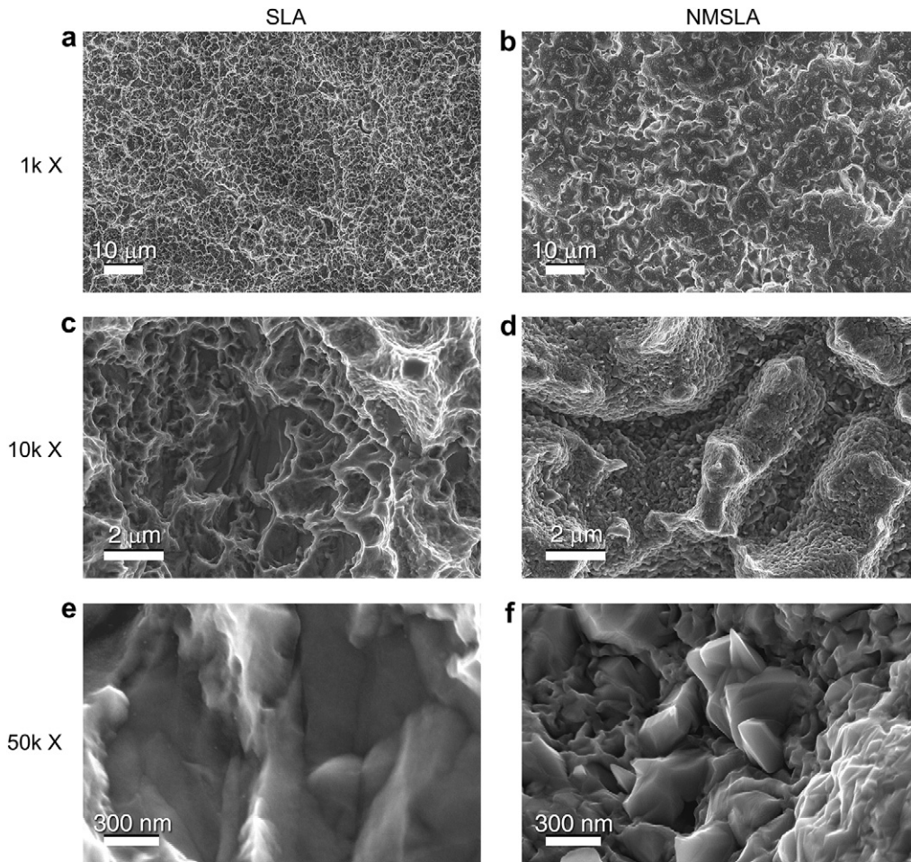
Fig. 3. SEM images of starting SLA samples (a,c,e), and of NMSLA samples (b,d,f) generated via oxidation in flowing synthetic air at 740 °C for 90 min. These images indicate that the NM process yielded a relatively high density of nanoscale structures over the entire specimen surface and did not appreciably affect the overall microscale roughness of the SLA surface.
