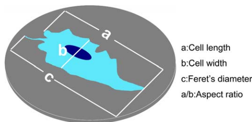
FIGURE 1. Cell morphology parameters: cell length (a), cell width (b), and Feret's diameter (c). [Color figure can be viewed in the online issue, which is available at wileyonlinelibrary.com .]
