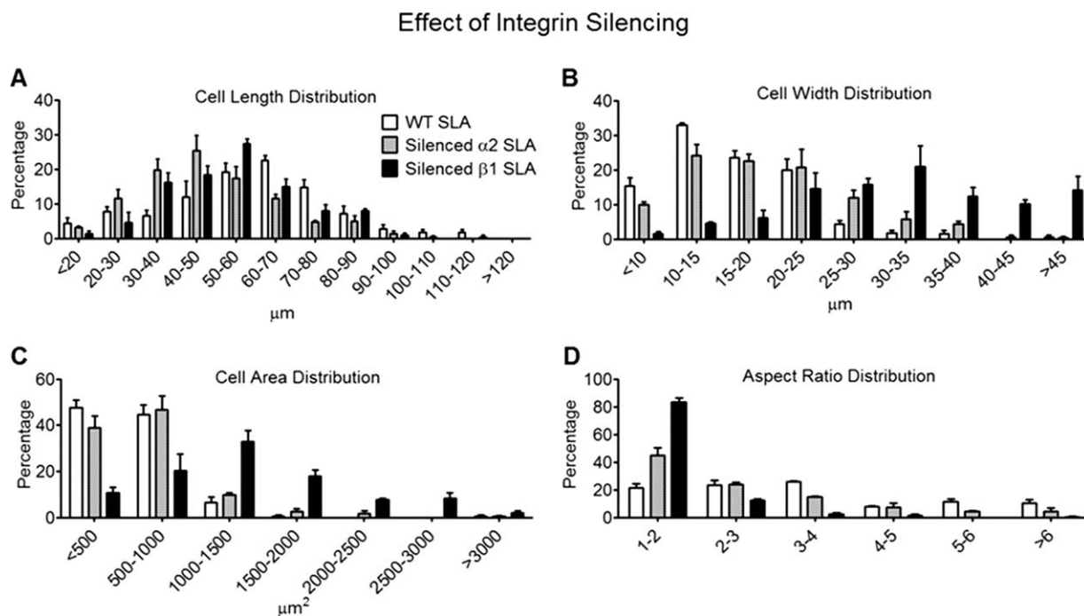
FIGURE 6. Cytomorphometric analyses of wild-type MG63 cells, \alpha 2 -silenced MG63 cells, and \beta 1 -silenced MG63 cells grown on SLA surfaces: cell length distribution (A), cell width distribution (B), cell area distribution (C), and aspect ratio distribution (D) ( n = 3 ).
